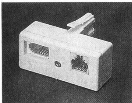
2407 BT PLUG TO U.S. & BT SOCKET X1 EACH -6P4C X 2 -6P6C X 2
