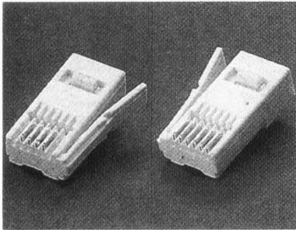
U.K. PLUG LEFT SIDE RIGHT SIDE 1161-6P4C 1160-6P4C -6P6C -6P6C
